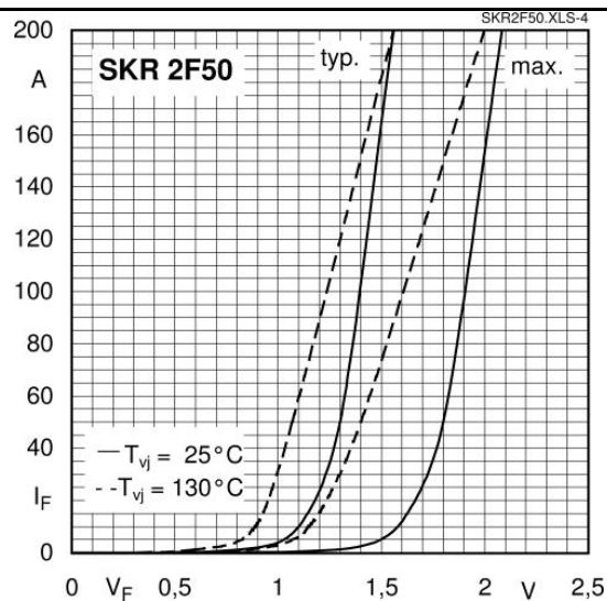
Fig. 4 Forward characteristics
