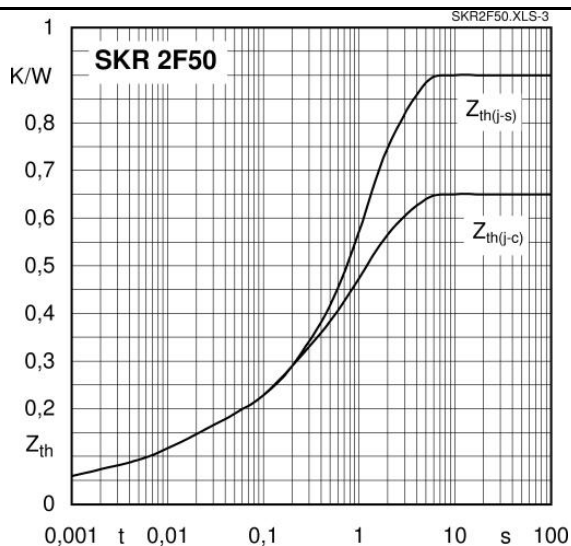
Fig. 3 Transient thermal impedance vs. time
