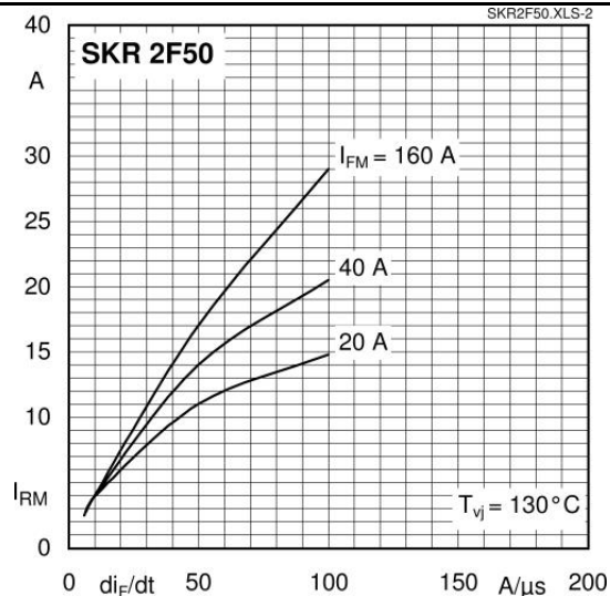
Fig. 2 Peak recovery current vs. current decrease
