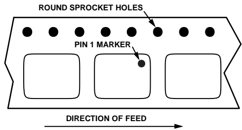
Figure 19. ADM6339 Reel Orientation
