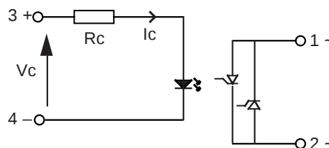
Figure 3 — LS relays
