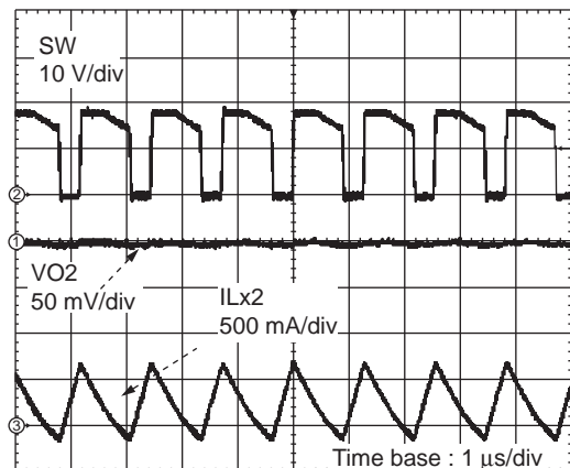
PWM Operation Discontinuous Mode VIN = 12 V, VS = 17.7 V, ILOAD = 10 mA
