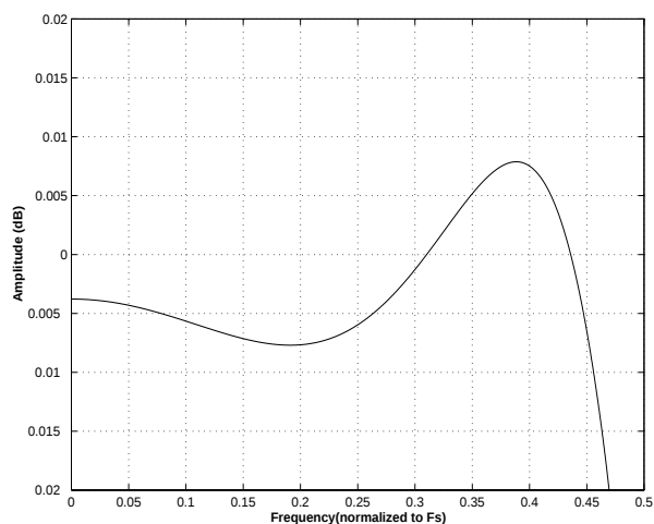
Figure 25. Single-Speed (fast) Passband Detail
