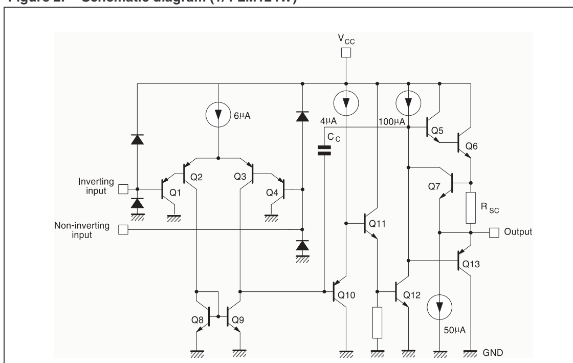
Figure 2. Schematic diagram (1/4 LM124W)
