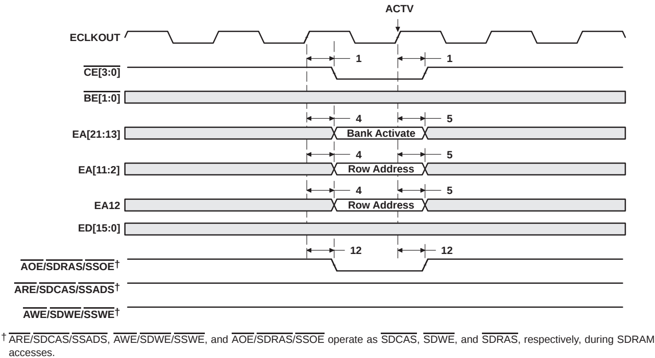
Figure 34. SDRAM ACTV Command
