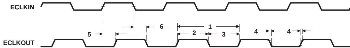
Figure 27. ECLKOUT Timings
