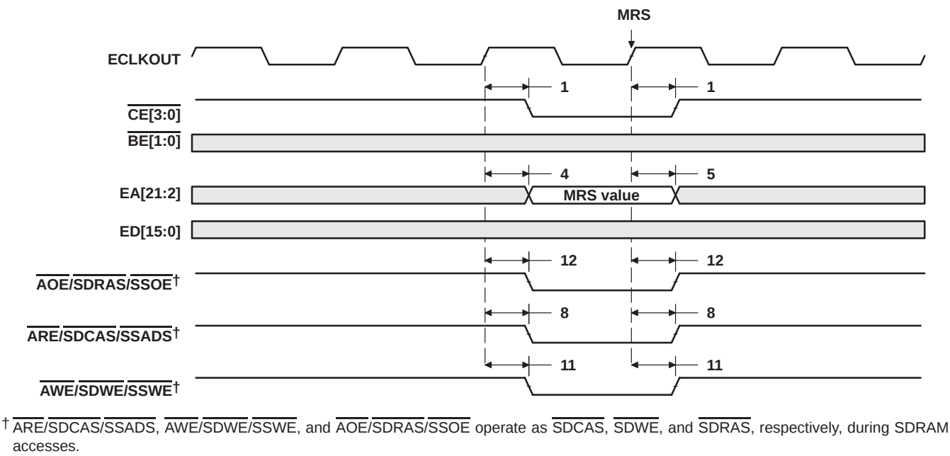
Figure 38. SDRAM MRS Command
