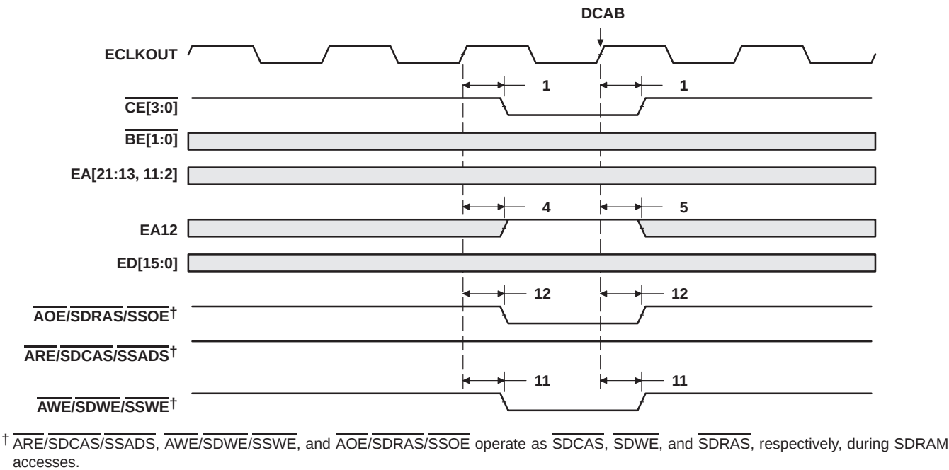
Figure 35. SDRAM DCAB Command
