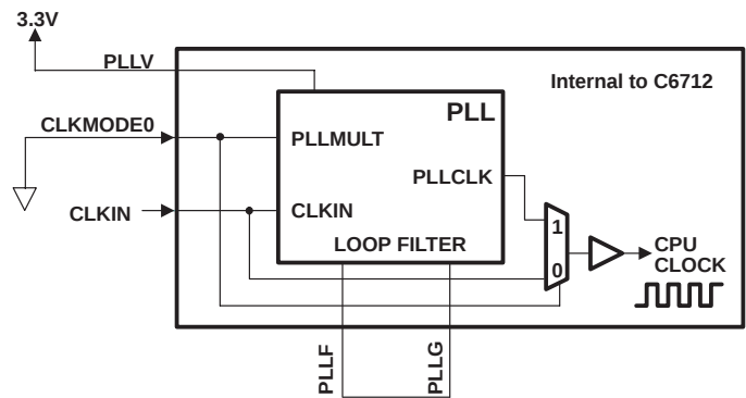
Figure 9. External PLL Circuitry for x1 (Bypass) Mode Only [C6712]
