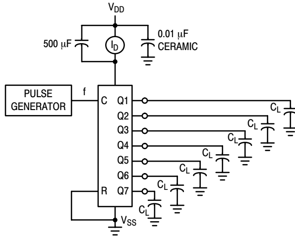
Figure 3. Power Dissipation Test Circuit
