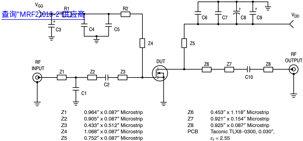
Figure 1. MRF21010L Test Circuit Schematic
