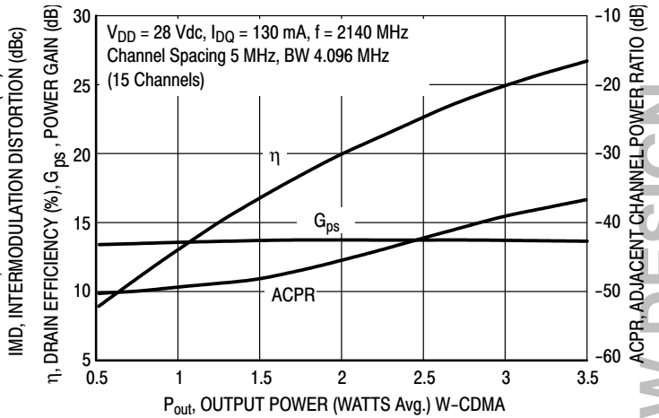
Figure 5. W-CDMA ACPR, Power Gain and Drain Efficiency versus Output Power
