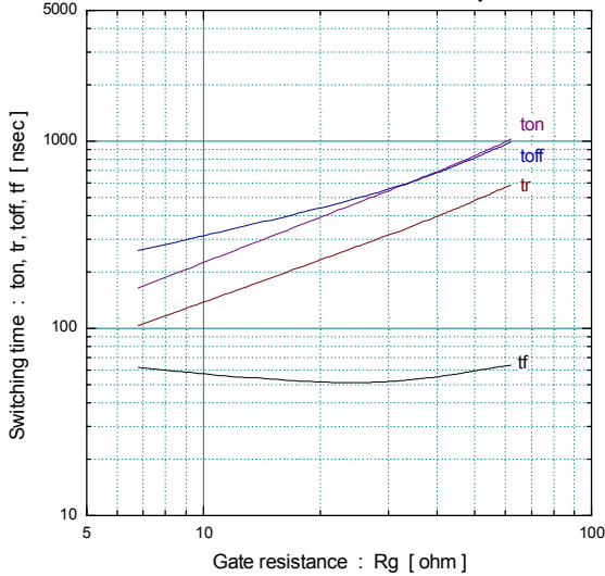
[ Inverter ] Switching time vs. Gate resistance (typ.) Vcc=300V, Ic=150A, VGE=+-15V, Tj= 25C
