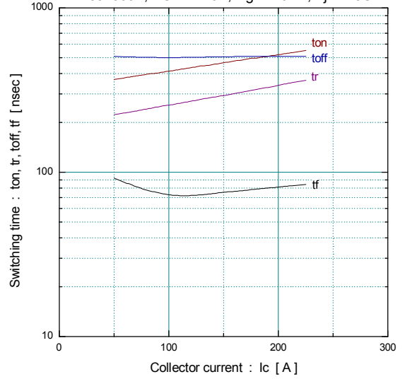
[ Inverter ] Switching time vs. Collector current (typ.) Vcc=300V, VGE=+-15V, Rg= 24ohm, Tj= 125C
