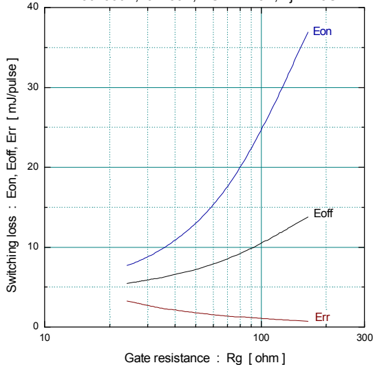
[ Inverter ] Switching loss vs. Gate resistance (typ.) Vcc=300V, Ic=150A, VGE=+-15V, Tj= 125C
