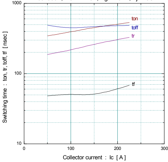
[ Inverter ] Switching time vs. Collector current (typ.) Vcc=300V, VGE=+-15V, Rg=24ohm, Tj= 25C
