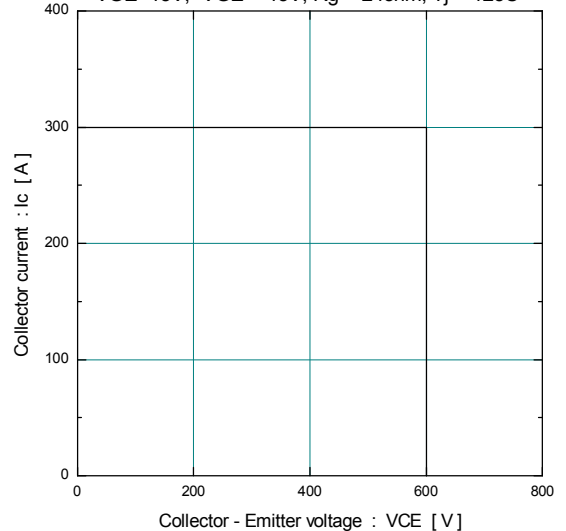
[ Inverter ] Reverse bias safe operating area +VGE=15V, -VGE<=15V, Rg>=24ohm, Tj<=125C
