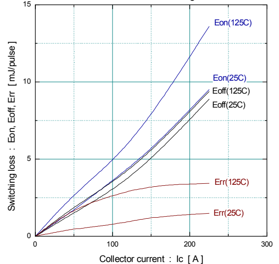
[ Inverter ] Switching loss vs. Collector current (typ.) Vcc=300V, VGE=+-15V, Rg=24ohm
