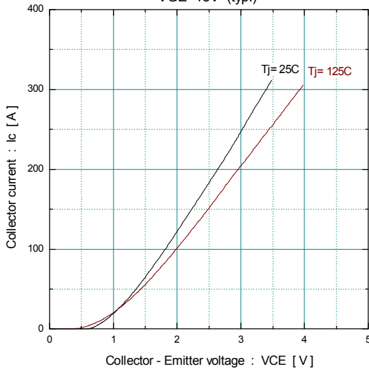
Collector current vs. Collector-Emitter voltage VGE=15V (typ.)
