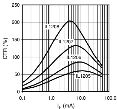
Fig. 12 - CTR vs. I_F Saturated, ( V_{CE} = 0.4\text{ V} , T_{amb} = 25\text{ °C} )
