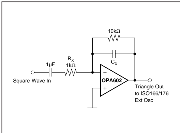
FIGURE 2. Square-Wave to Triangle Wave Signal Conditioner for Driving ISO176 Ext Osc Pin.
