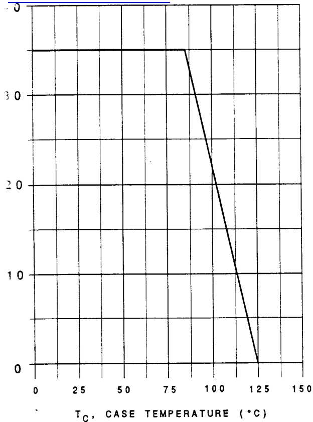
4S ON-STATE CURRENT vs. CASE TEMPERATURE
