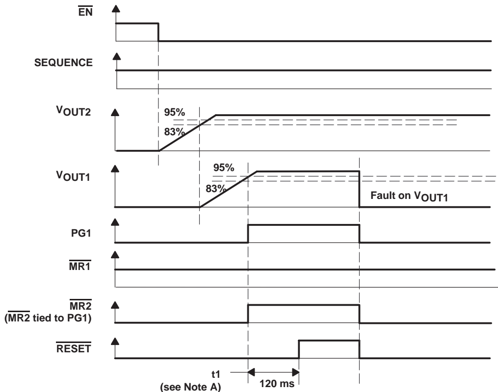
Figure 29. Timing When a Fault Occurs on V_{OUT1}
