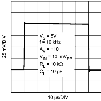
Small Signal Step Response, A_V = 10
