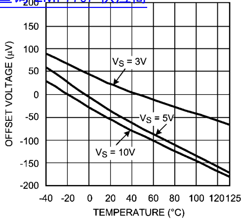
Offset Voltage vs. Temperature 查询"LMP7707"供应商
