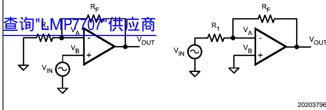
FIGURE 8. Op Amp with Resistive Feedback. (a) Non-inverting (b) Inverting
