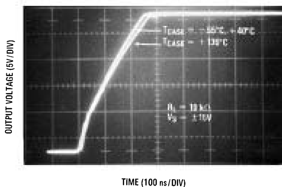
Step Response
