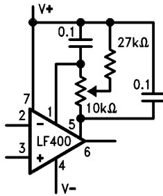
FIGURE 4a. V_{OS} Adjust Circuit
