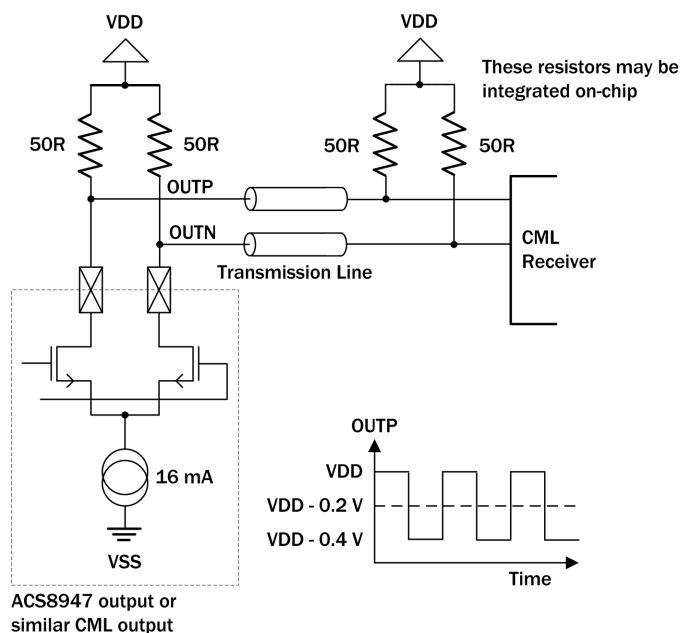
Figure 13 CML Output - DC Coupled to CML Receiver
