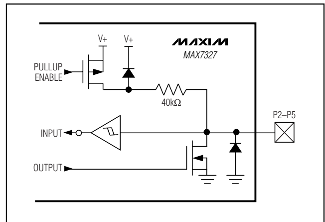
Figure 11. MAX7327 Open-Drain I/O Port Structure
