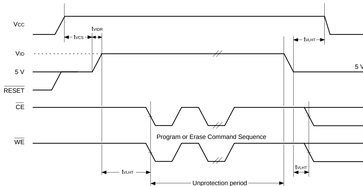
Figure 13 Temporary Sector Unprotection Timing Diagram
