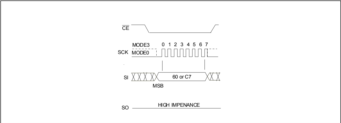
Figure 19: Chip Erase Sequence
