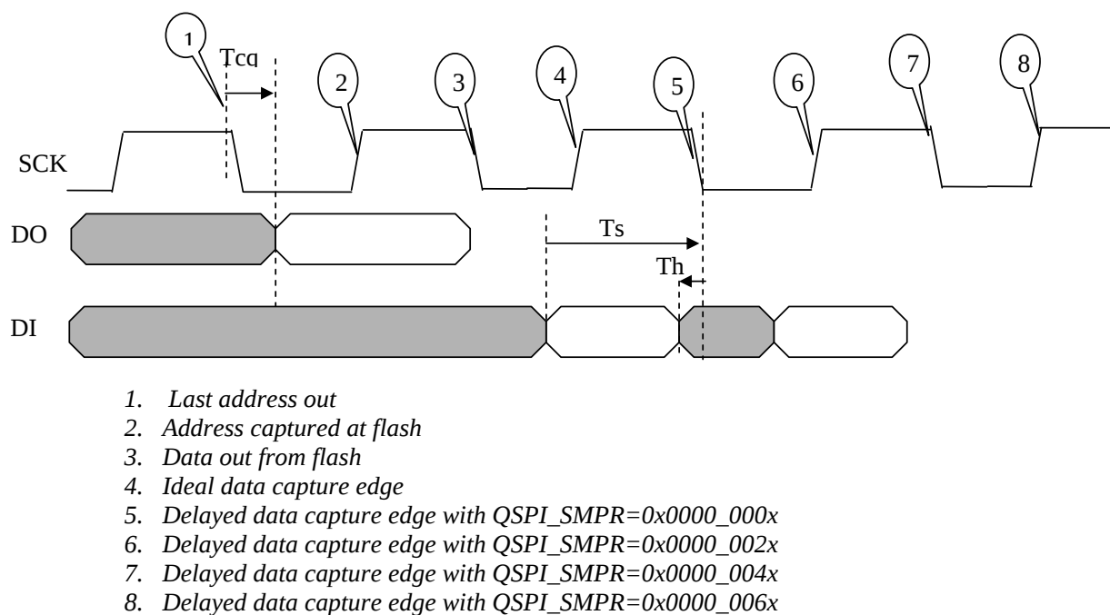
Figure 46. QuadSPI input timing diagram
