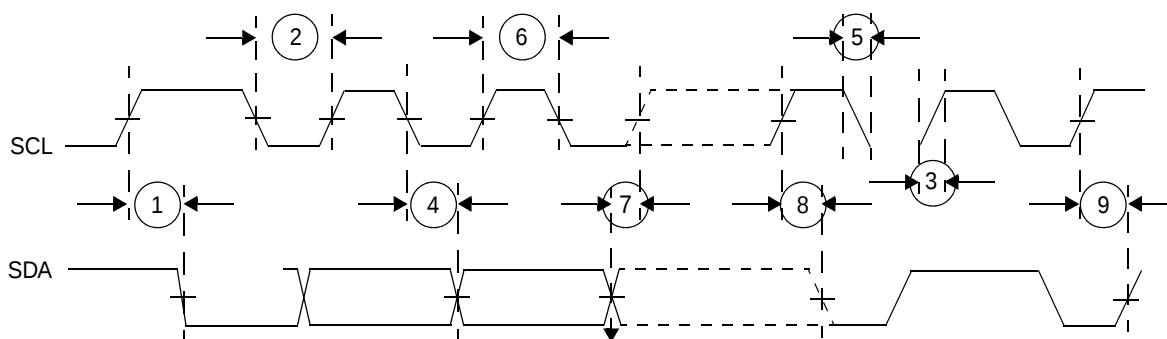
Figure 44. I²C input/output timing
