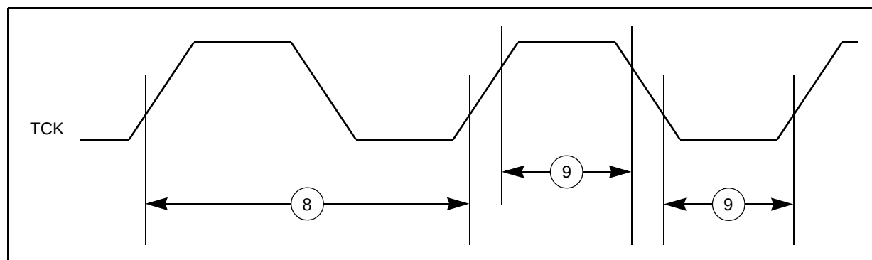
Figure 29. Nexus TCK timing
