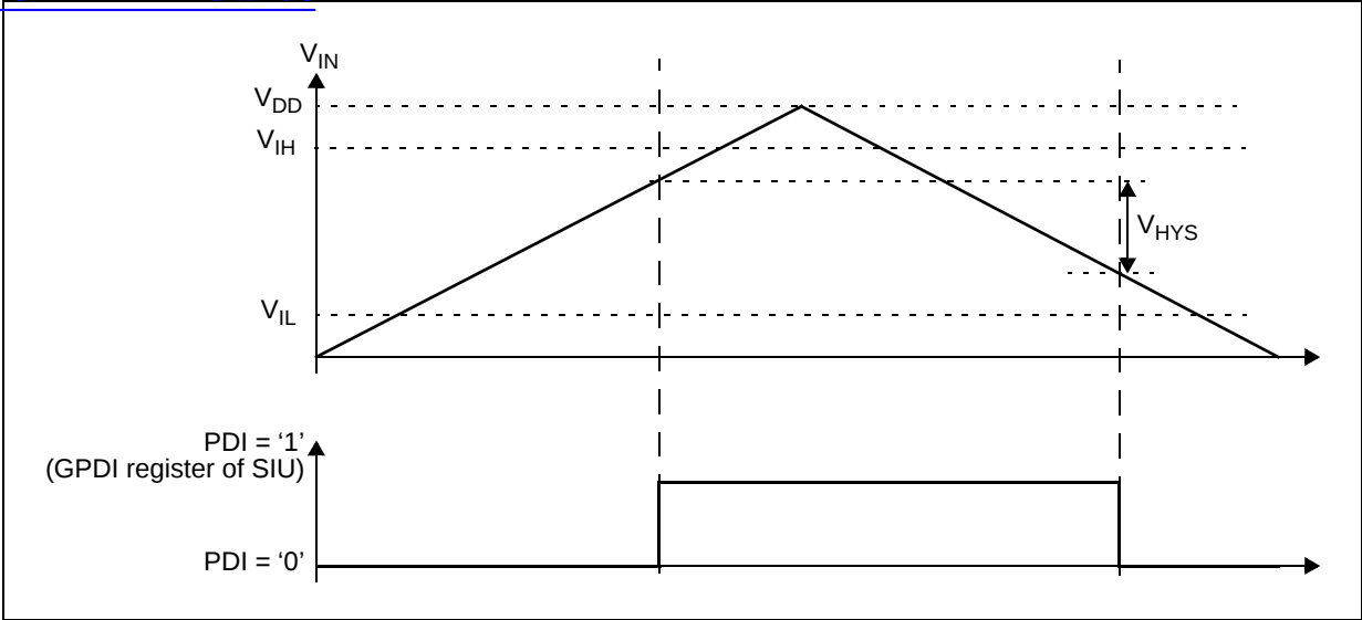
Figure 12. I/O Input DC electrical characteristics definition
