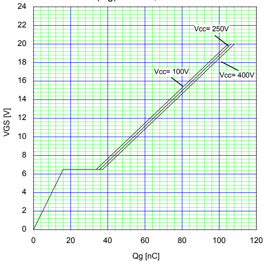
Typical Gate Charge Characteristics V_{GS} = f(Q_g) : I_D = 21 A, T_{ch} = 25^\circ C
