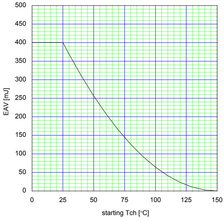
Maximum Avalanche Energy vs. starting Tch E(AV)=f(\text{starting Tch}):V_{CC}=50V, I(AV)\leq 21A
