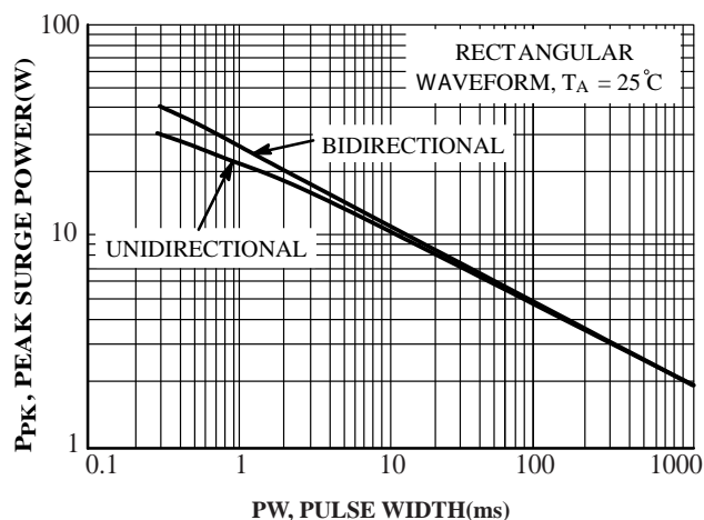
FIG.7 Maximum Non-repetitive Surge Power, P_{PK} Versus PW
