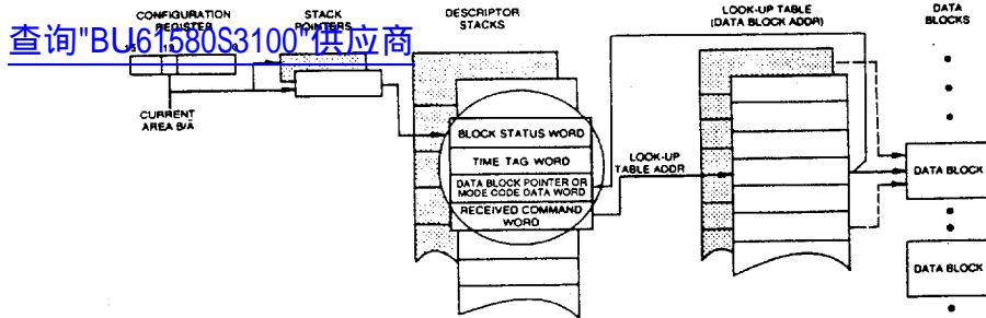
FIGURE 27. RT MEMORY MANAGEMENT: SINGLE MESSAGE MODE
