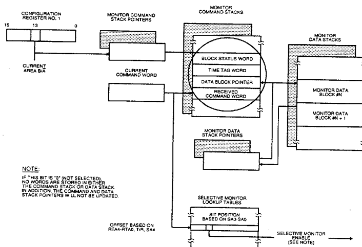
FIGURE 31. SELECTIVE MESSAGE MONITOR MEMORY MANAGEMENT
