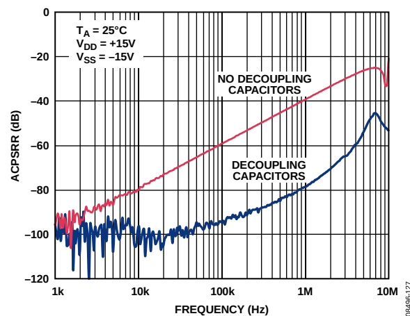
Figure 26. ACPSRR vs. Frequency
