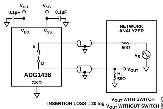
Figure 35. Insertion Loss
