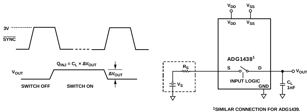
Figure 32. Charge Injection
