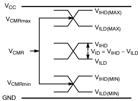
Figure 9. V_{CM} Diagram
