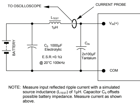
Figure 15. Input Reflected Ripple Current Test Setup.
