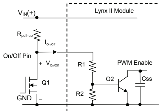
Figure 21. Circuit configuration for using negative logic On/Off
