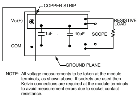
Figure 16. Output Ripple and Noise Test Setup.
