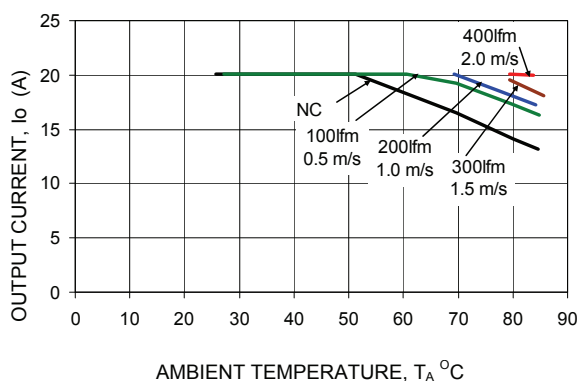
Figure 14. Derating Output Current versus Local Ambient Temperature and Airflow ( V_{in} = 3.3Vdc , V_o=1.8Vdc ).
