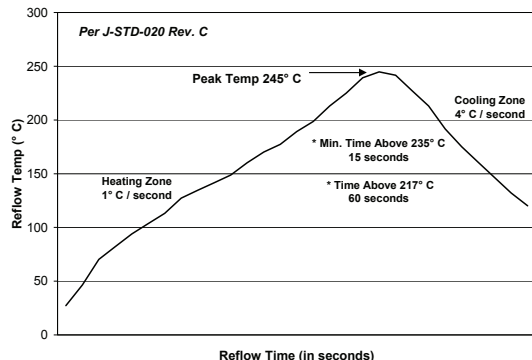
Figure 30. Recommended linear reflow profile using Sn/Ag/Cu solder.
