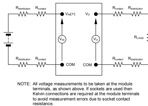
Figure 17. Output Voltage and Efficiency Test Setup.
