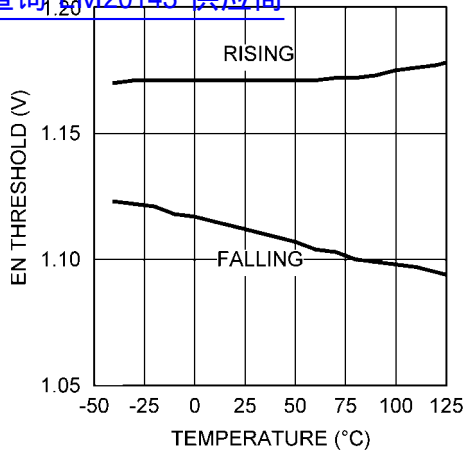
Enable Threshold vs. Temperature 查询"LM20143"供应商
