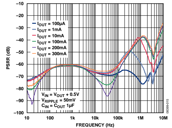
Figure 15. Power Supply Rejection Ratio vs. Frequency, V_{OUT} = 2.8\text{ V} , V_{IN} = 3.3\text{ V}
