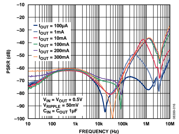
Figure 16. Power Supply Rejection Ratio vs. Frequency, V_{OUT} = 3.3\text{ V} , V_{IN} = 3.8\text{ V}
