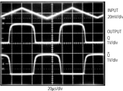
MAX912/MAX913 RESPONSE
