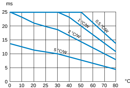
Thermal curves
