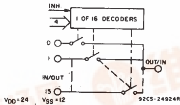
Fig. 1 – CD4067 functional diagram.
