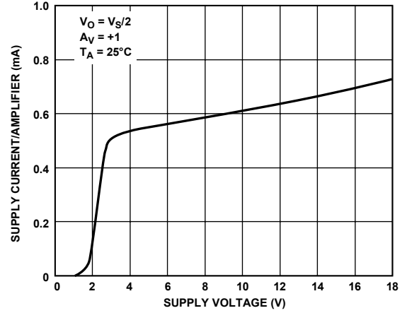
Figure 9. Supply Current/Amplifier vs. Supply Voltage
