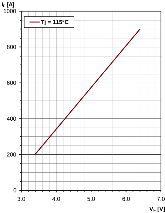
Fig. 9 Diode on-state voltage characteristics
