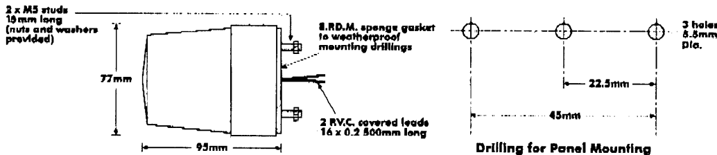
Drilling for Panel Mounting
