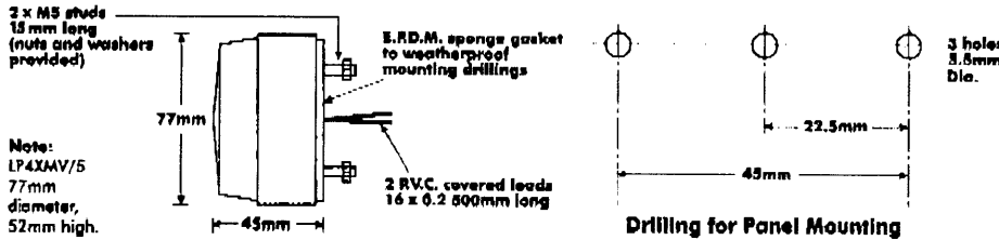
Drilling for Panel Mounting
