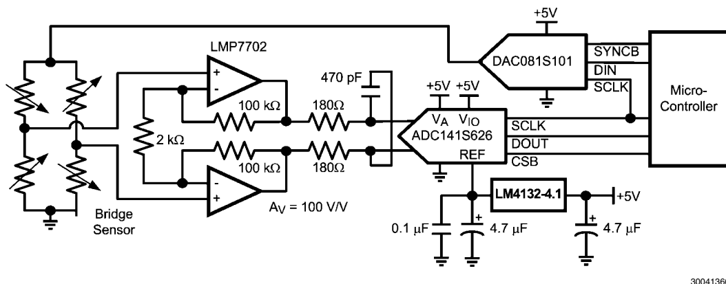
FIGURE 13. Interfacing the ADC141S626 to a Bridge Sensor
