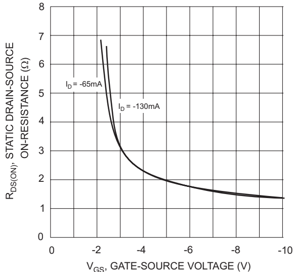
R_{DS(on)} , STATIC DRAIN-SOURCE ON-RESISTANCE (Ω) V_{GS} , GATE-SOURCE VOLTAGE (V) Fig. 5, Static Drain-Source On-Resistance vs. Gate-Source Voltage
