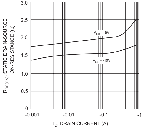
R_{DS(on)} , STATIC DRAIN-SOURCE ON-RESISTANCE (Ω) I_D , DRAIN CURRENT (A) Fig. 4, Static Drain-Source On-Resistance vs. Drain Current
