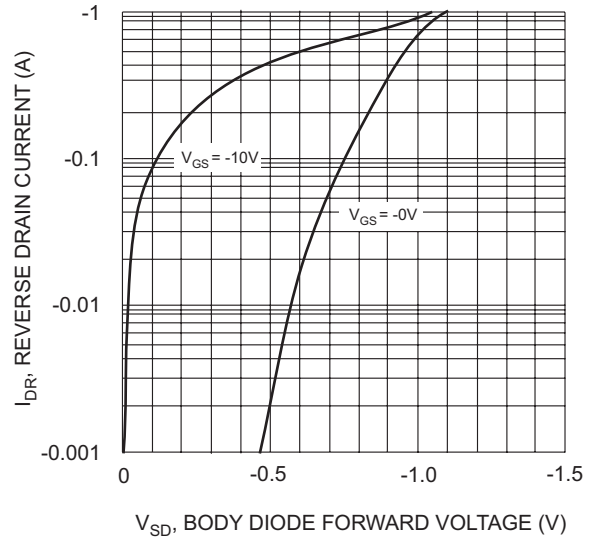
I_{DR} , REVERSE DRAIN CURRENT (A) V_{SD} , BODY DIODE FORWARD VOLTAGE (V) Fig. 6, Reverse Drain Current vs. Body Diode Forward Voltage
