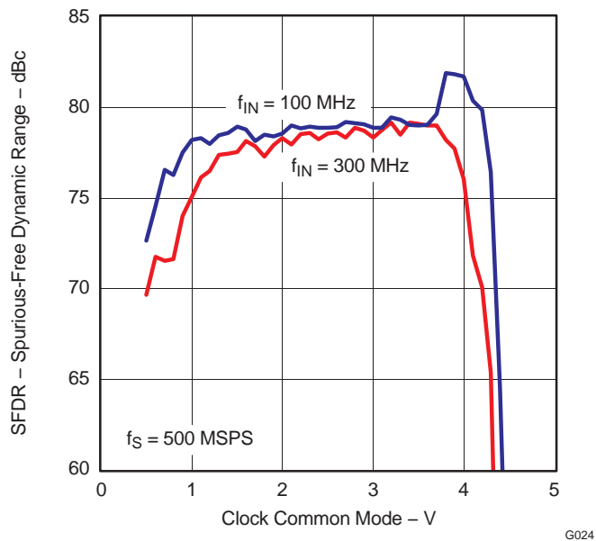
Figure 62. ADS5463 SFDR versus Clock Common Mode
