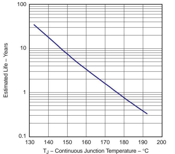
Figure 69. Operating Life Derating Chart, Wirebound Voiding Fail Mode
