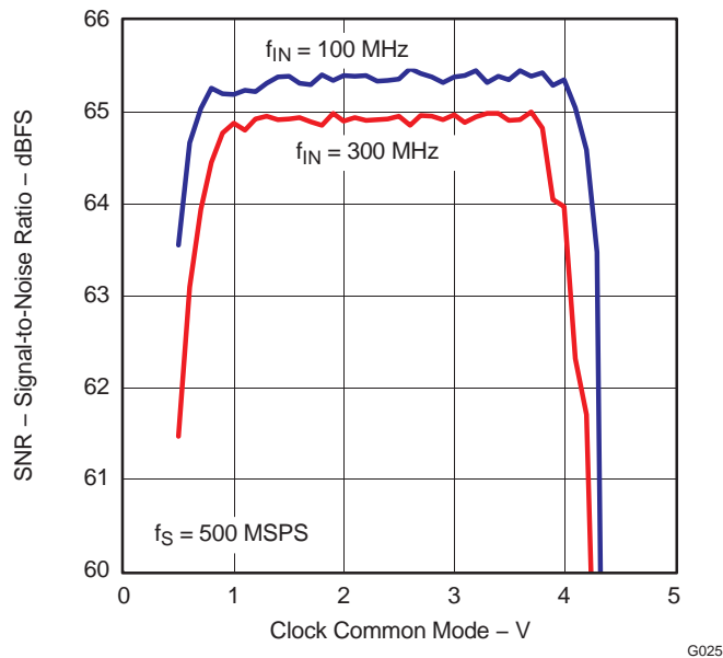
Figure 63. ADS5463 SNR versus Clock Common Mode
