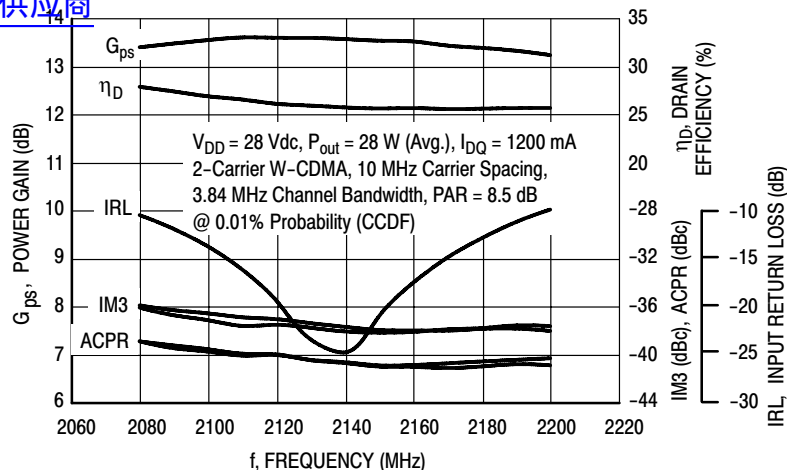
Figure 3. 2-Carrier W-CDMA Broadband Performance @ P_{out} = 28 \text{ Watts Avg.}
