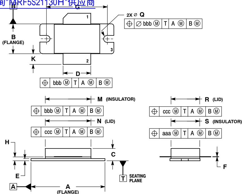
CASE 465B-03 ISSUE D NI-880 MRF5S21130HR3
