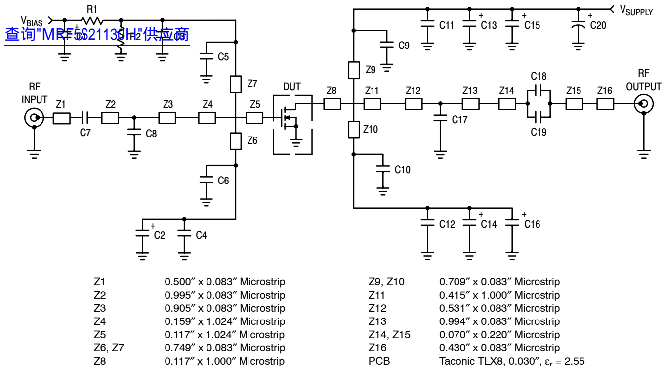
Figure 1. MRF5S21130HR3(SR3) Test Circuit Schematic
