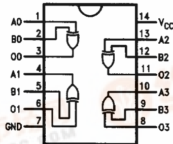
Dual-In-Line Package
