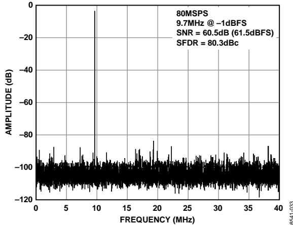
Figure 4. AD9609-80 Single-Tone FFT with f_{IN} = 9.7 MHz
