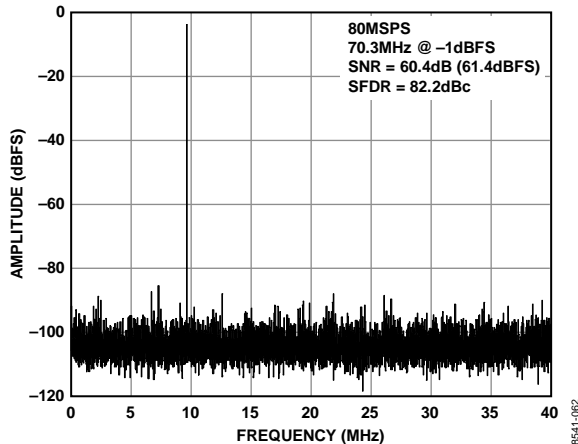
Figure 5. AD9609-80 Single-Tone FFT with f_{IN} = 70.3 MHz
