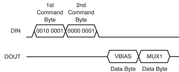
Figure 60. Read from Register
