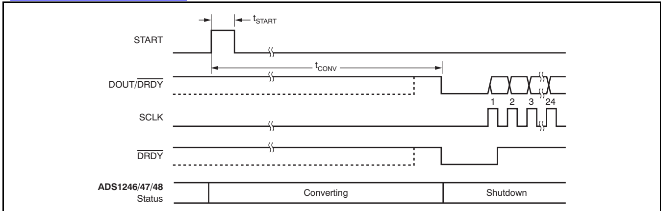
Figure 47. Timing for Single Conversion Using START Pin
