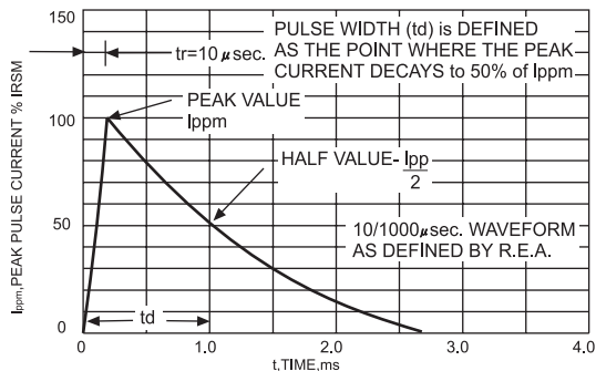
FIG.3-PULSE WAVEFORM
