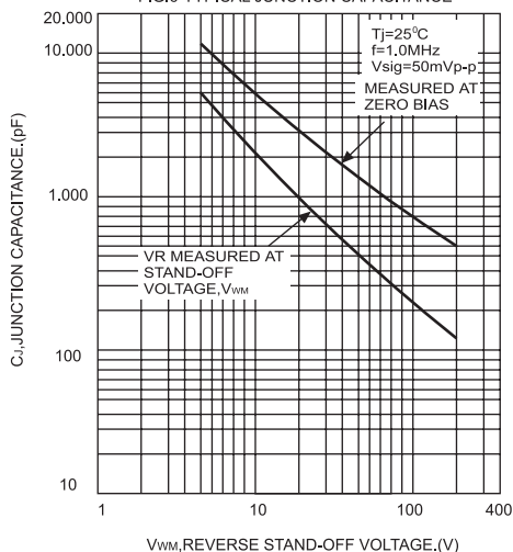
FIG.6-TYPICAL JUNCTION CAPACITANCE
