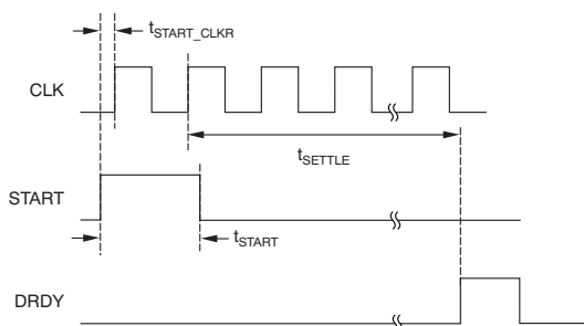
Figure 3. START Timing
