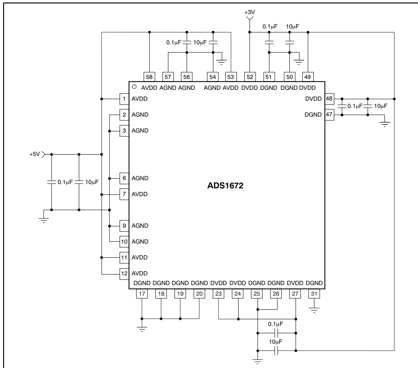
Figure 39. Power-Supply Decoupling
