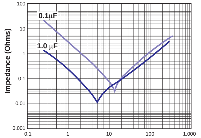
Figure 12. Impedance vs Frequency for Z5U Dielectric
