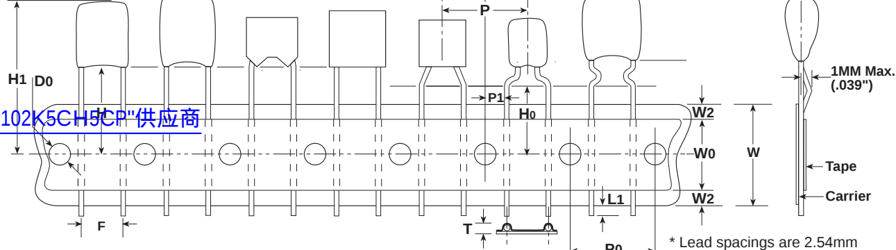
Figure 2: Lead Tape Configuration (See Table Below)
