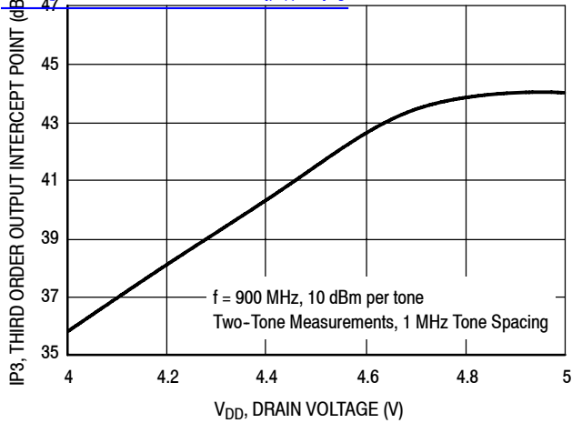
Figure 8. Third Order Output Intercept Point versus Drain Voltage
