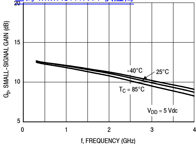
Figure 2. Small-Signal Gain (S21) versus Frequency
