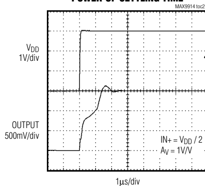
POWER-UP SETTLING TIME
