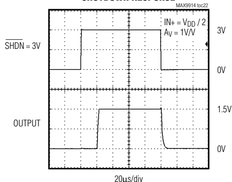
SHUTDOWN RESPONSE
