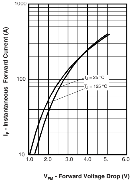
Fig. 11 - Typical Forward Voltage Drop vs. Instantaneous Forward Current
