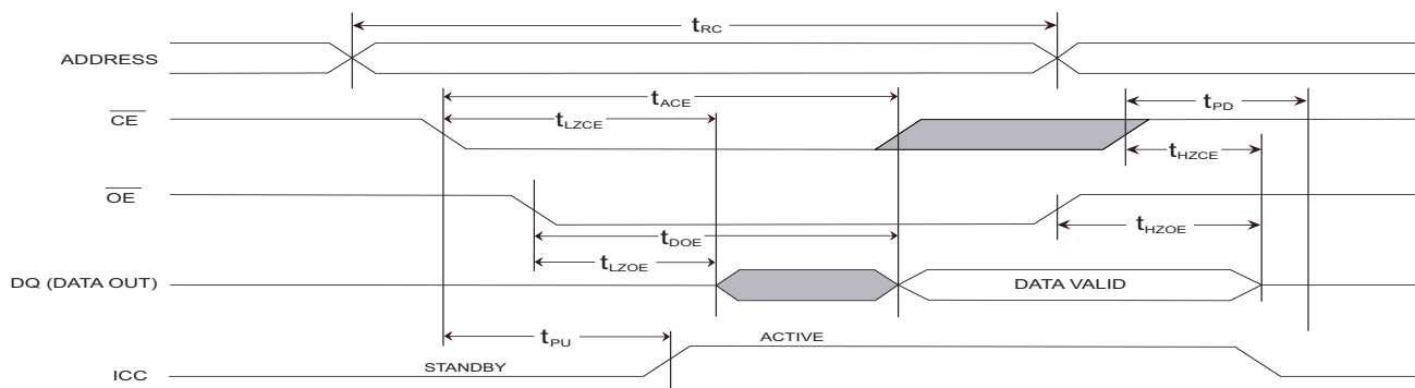
Figure 6. SRAM Read Cycle 2: \overline{\text{CE}} Controlled [4,14]
