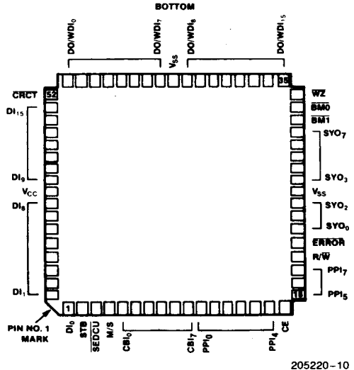
Figure 8a. 8206 Leadless Chip Carrier (LCC) Pinout Diagram
