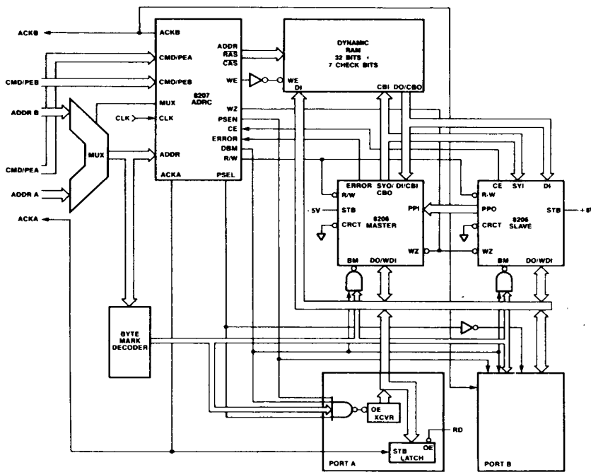
Figure 6. Dual Port RAM Subsystem with 8206/8207 (32-bit bus)
