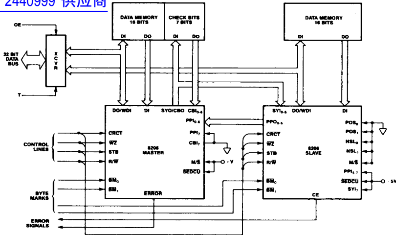
Figure 5. 32-Bit 8206 System Interface
